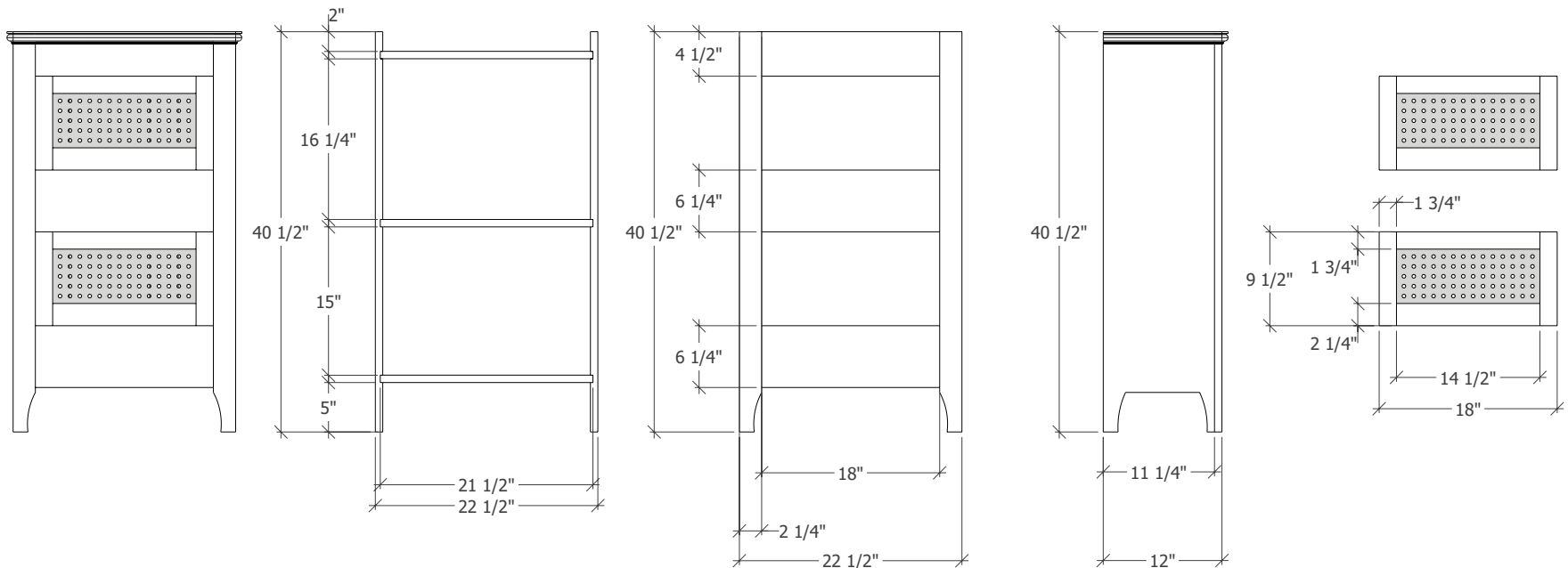
Side view of completed cabinet
