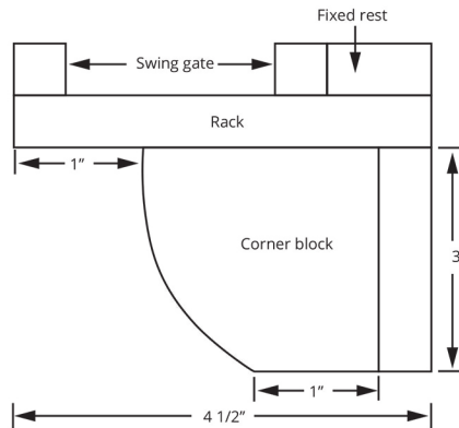
Fig. 4 - Rack Support (Side View) (Not to scale)
