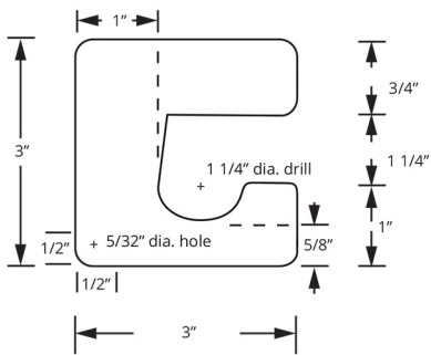
Fig. 2 - Swing Gate
