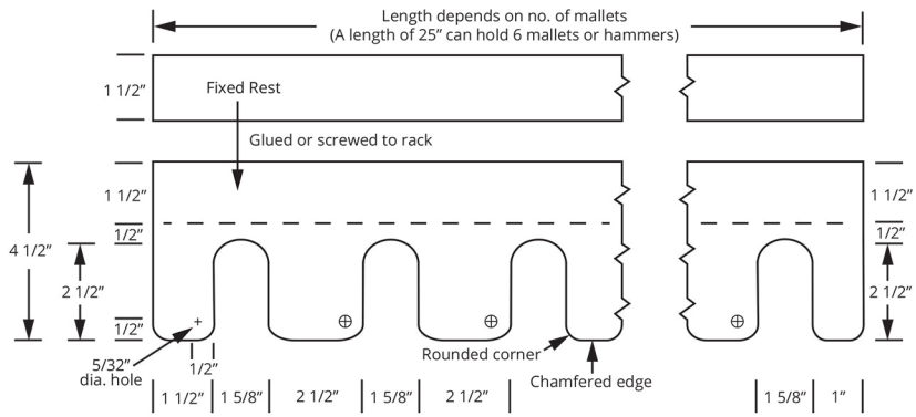
Fig. 1 - Rack Body
