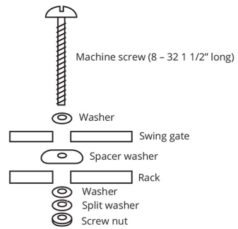
Fig. 3 - Hardware Installation
